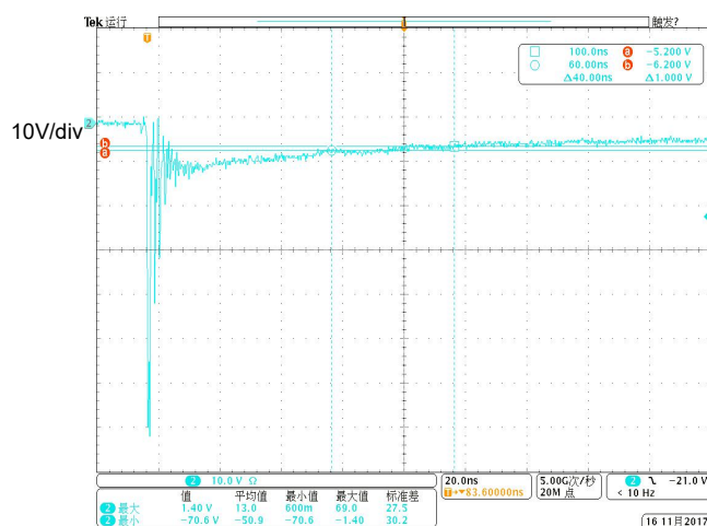
20ns/div Fig 8. ESD clamping voltage (IEC61000-4-2-8KV contact)
